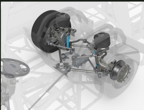
Independent Front Axle
